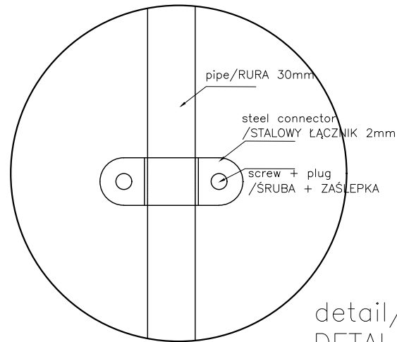
detail/ DETAL 02
