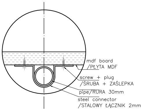
detail/ DETAL 03
