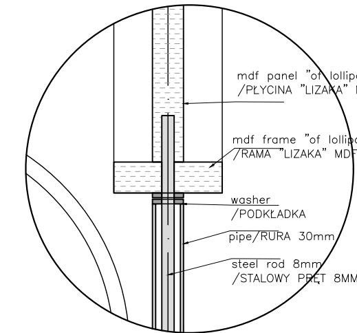
detail/ DETAL 01
