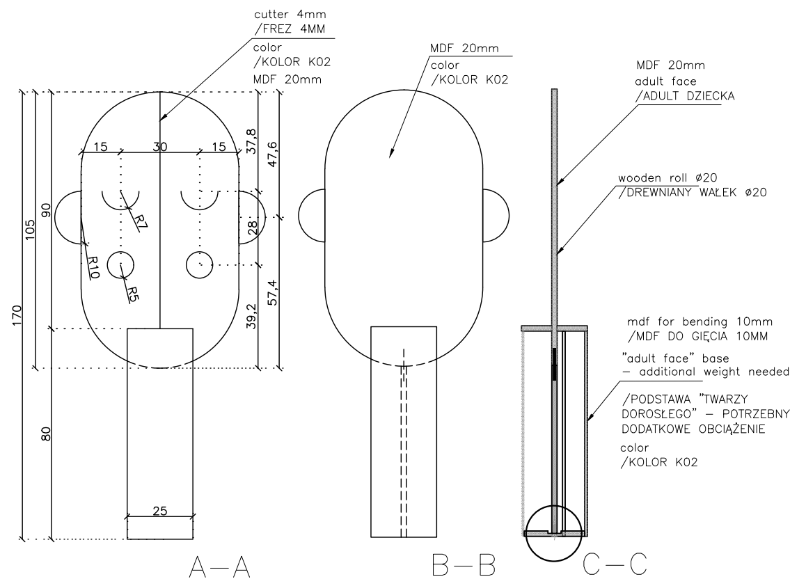
detail/ DETAL 01
